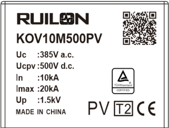
KOV10M500PV 标识 Marking
