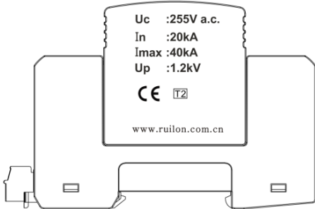
TA40-255N 标识 Marking
