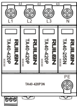
通信标识 Communication marking
