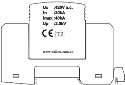
TA40-420P 标识 Marking
